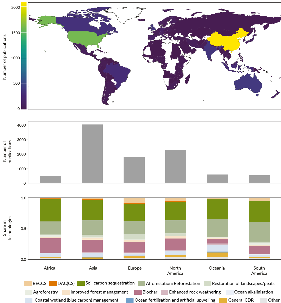
Figure 2.4. The distribution of place-based Carbon Dioxide Removal (CDR) research is very uneven across major global regions. Total number of CDR research publications that mention a geographic location in abstract or title, shown by country (top) and world region (middle). Share of CDR methods in scientific research publication that refer to a specific geographic location, shown by world region (bottom). Definitions: Bioenergy with Carbon Capture and Storage (BECCS), Direct Air Carbon Capture (DAC) and Direct Air Carbon Capture and Storage (DACCS).
